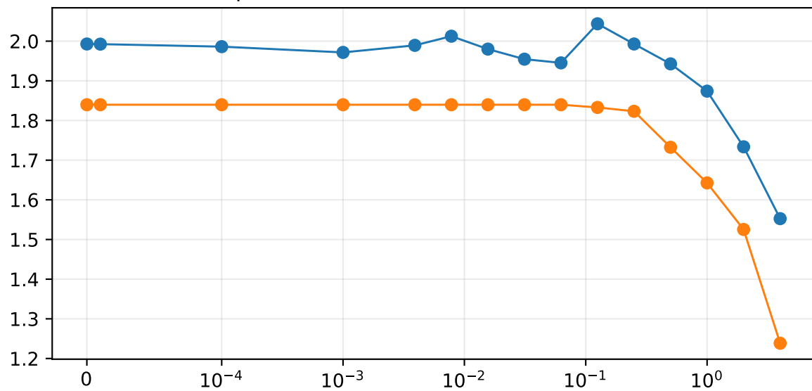
Good-state Sharpe
